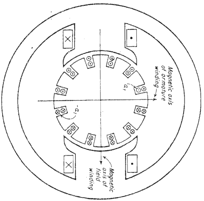
Fig. 3-19. Cross section of a 2-pole d-c machine.
